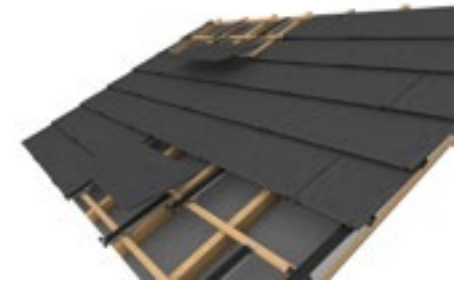
3 Insert MATCH Slate modules
