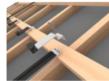
2 The rail hooks are mounted directly on the roof battens.
