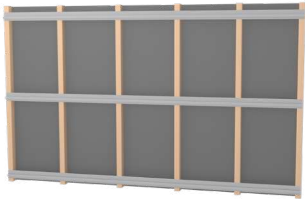
1 Apply transverse profiles to the vertical structure of the building.
